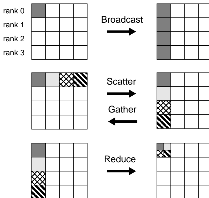
Figure 5: Primitive Collective Operations
