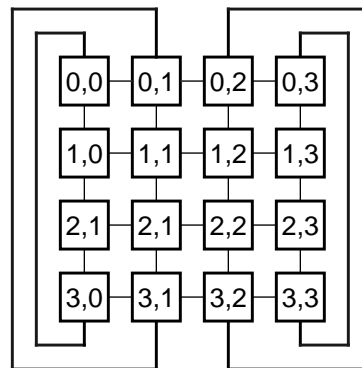
Figure 7: 2D Cartesian Topology
